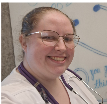
Janaye Mattice
